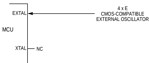
Figure 2-9. External Oscillator Connections
