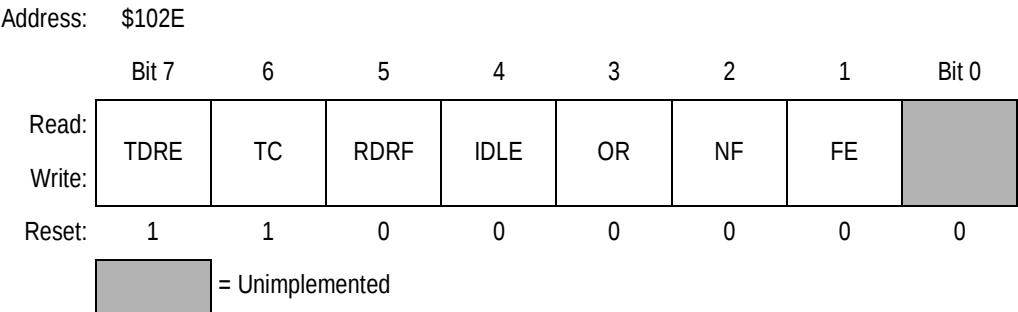
Figure 7-6. Serial Communications Status Register (SCSR)
