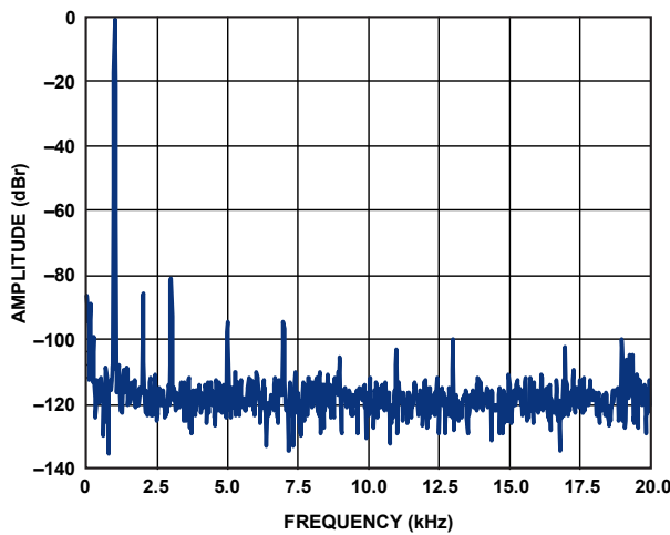
Figure 74. FFT, -1 dBFS, Analog In → ADC → DAC → Line Out
