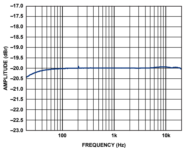
Figure 17. Frequency Response, 8 Ω + 33 μH, Analog In → Speaker Out
