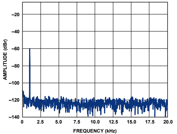
Figure 18. FFT, -60 dBFS, Analog In → Headphone Out
