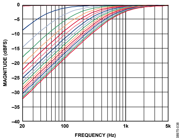
Figure 105. Post-HPF Frequency Response
