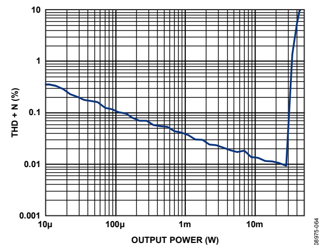
Figure 21. THD + N vs. Output Power, 32 \Omega , Analog In → Headphone Out
