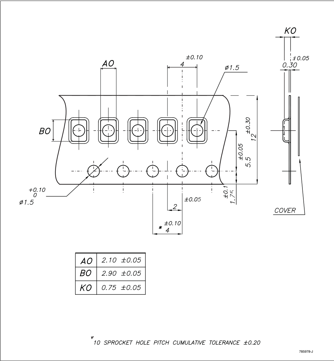
Figure 10. Carrier tape for QFN12 (2.2 x 1.5 x 0.5 mm) - 0.40 mm pitch
