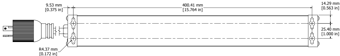
ASSEMBLY - VIEW FROM BOTTOM
