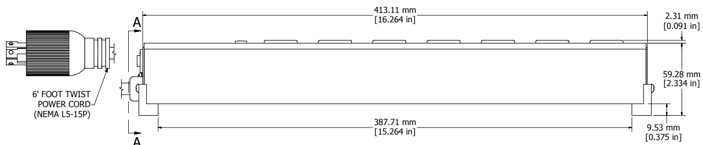
ASSEMBLY - VIEW FROM SIDE
