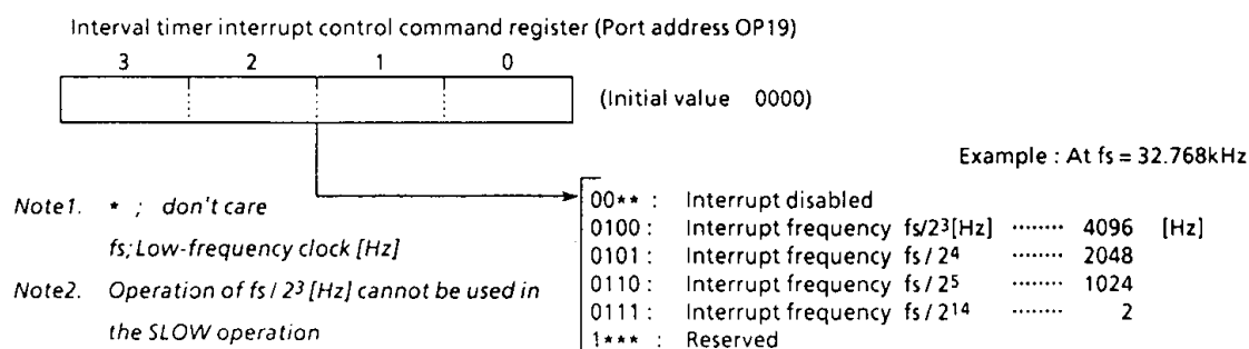
Figure 2-8. Command Register
