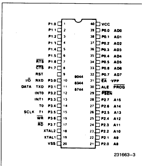
Figure 3A. DIP Pin Configuration
