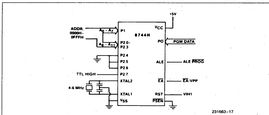
Figure 8. Programming Configuration
