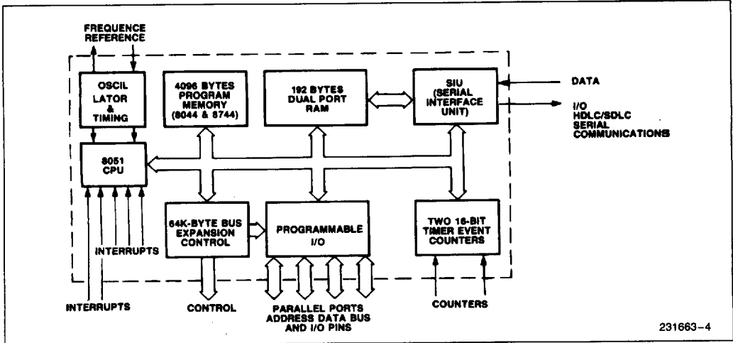
Figure 4. Block Diagram
