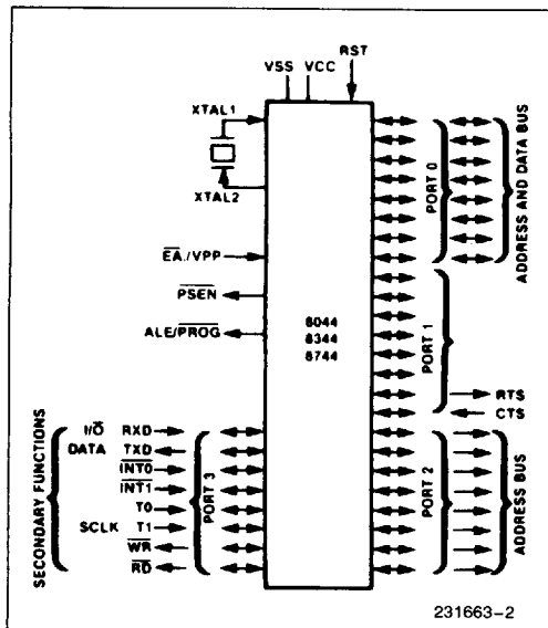
Figure 2. Logic Symbol
