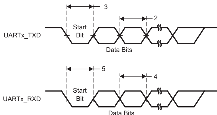
Figure 8-95. UART Timing
