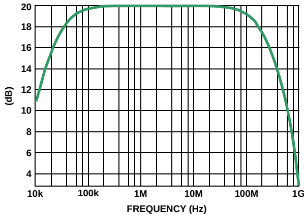
FIGURE 7. PREDICTED RESPONSE SHAPE TO V_{OUT} FOR A 50Ω SOURCE TO THE INPUT OF C1
