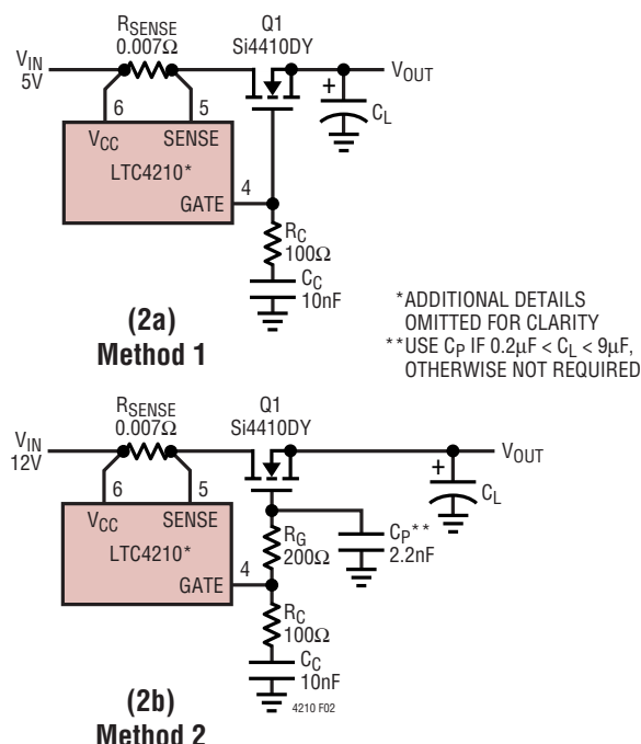
Figure 2. Frequency Compensation
