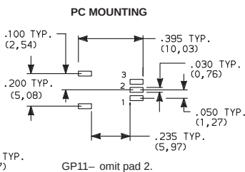
PC MOUNTING
