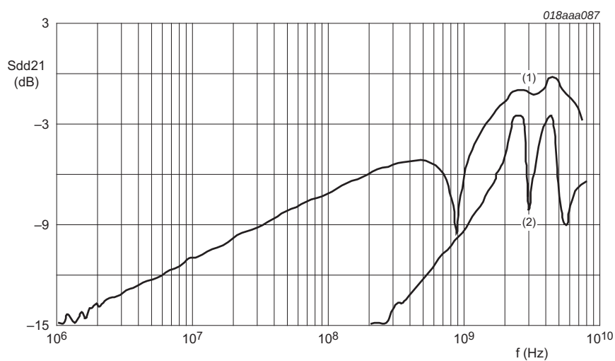
Fig 4. Mixed-mode differential and common-mode insertion loss; typical values
