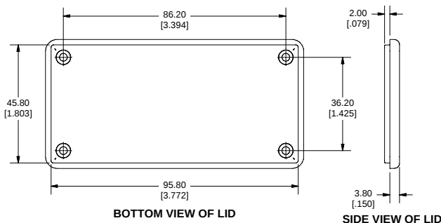
BOTTOM VIEW OF LID
