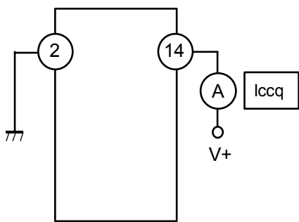
Test Circuit 3 Iccq
