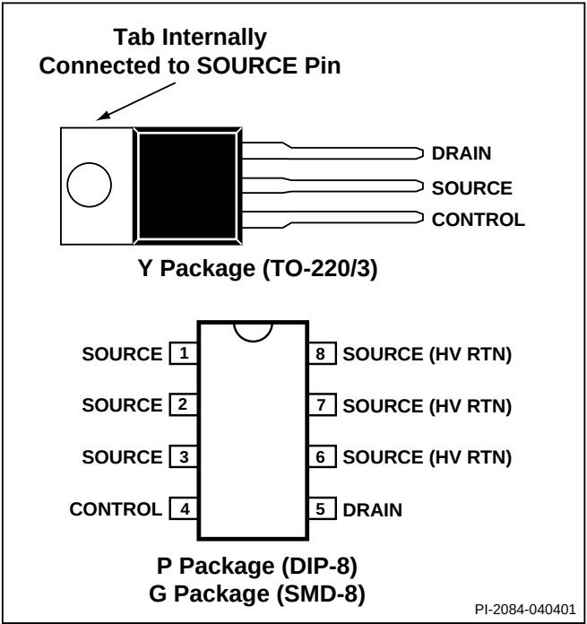
Figure 3. Pin Configuration.
