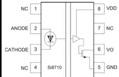
SOIC-8, DIP8, LGA8 Open Collector Output
