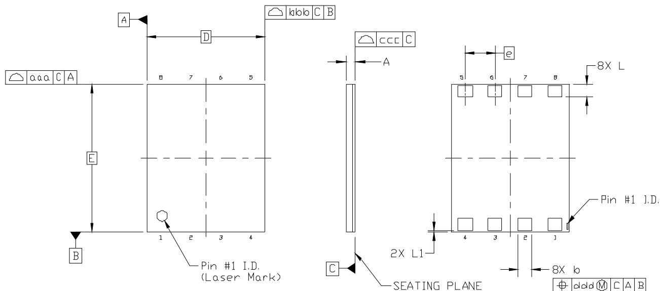
Figure 21. LGA8 Package
