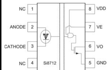
SOIC-8, DIP8, LGA8 Open Collector Output with Output Enable
