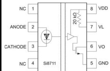
SOIC-8, DIP8, LGA8 Open Collector Output with 20 kΩ Pull-up Resistor
