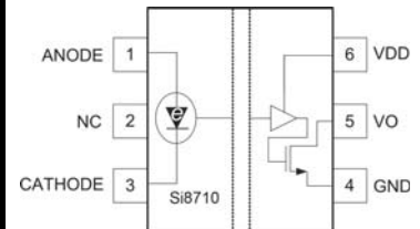
SDIP6 Open Collector Output
