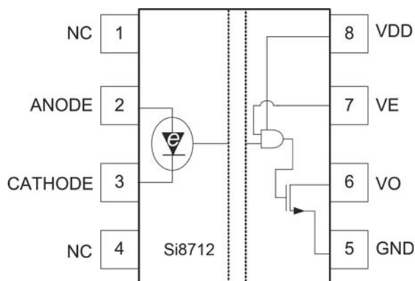
Figure 12. Pin Configuration
