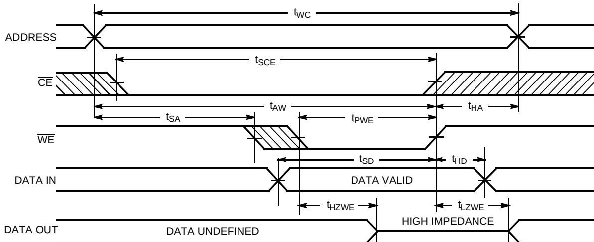
Write Cycle No.1 ( \overline{WE} Controlled) [11]
