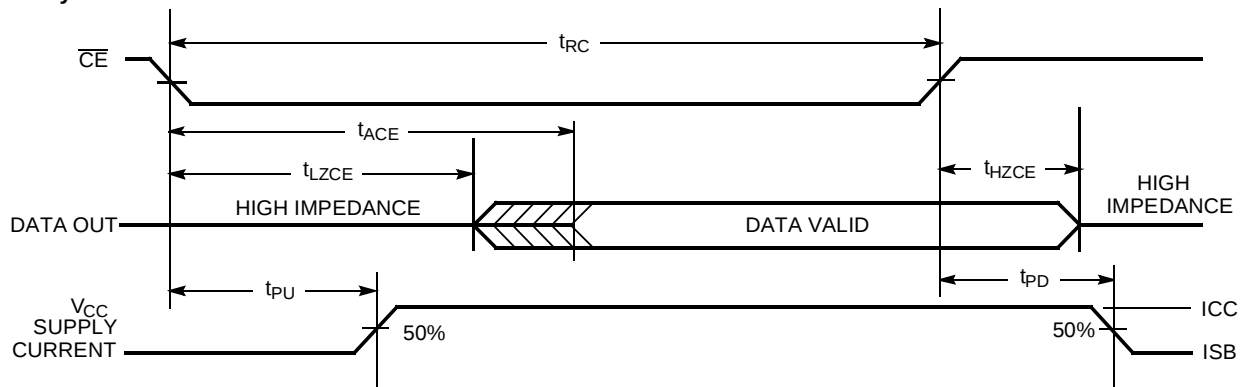
Read Cycle No.2 [12]
