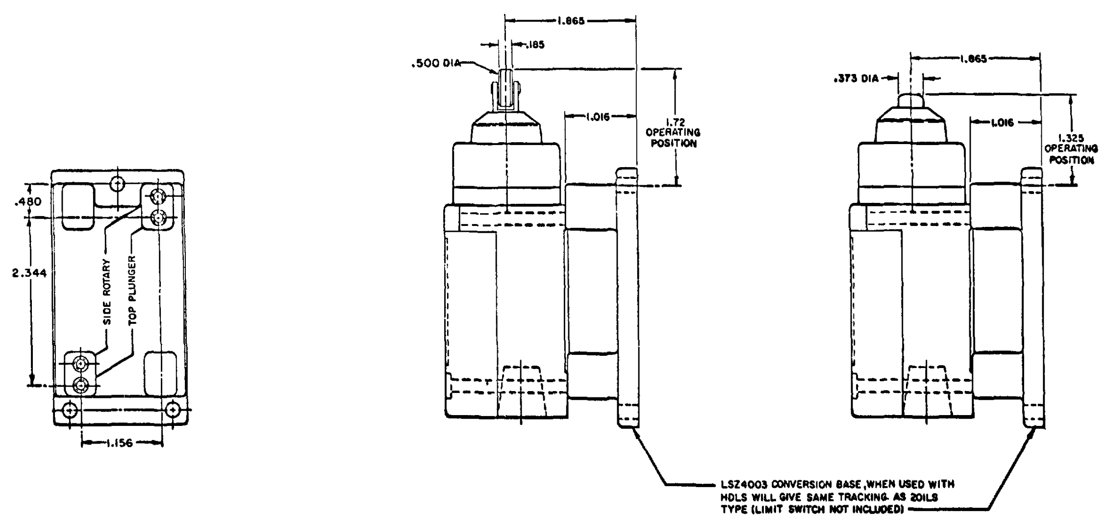
SINGLE POLE TOP PLUNGER LSZ4003
