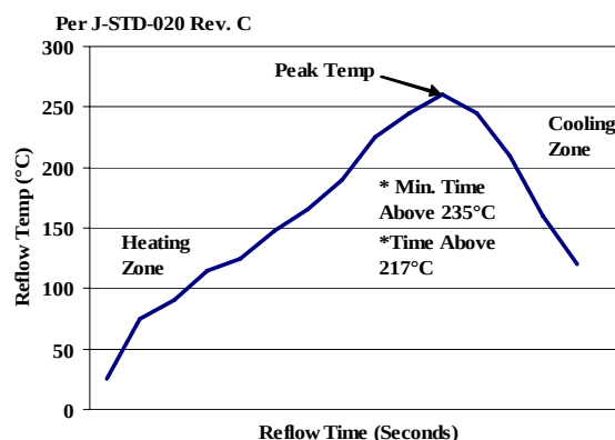
Figure 53. Recommended linear reflow profile using Sn/Ag/Cu solder.
