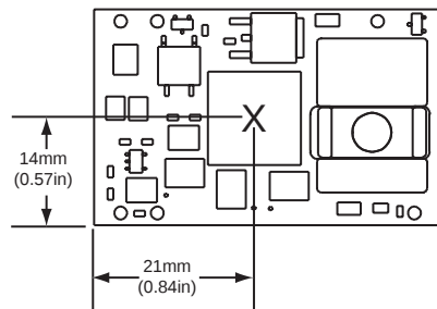
Figure 49. Pick and Place Location.
