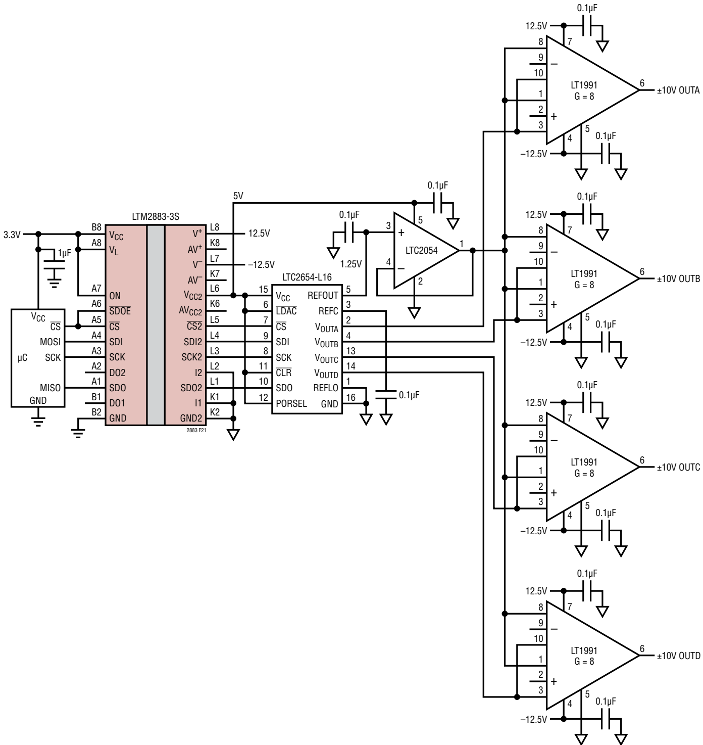
Figure 21. Quad 16-Bit ±10V Output Range DAC
