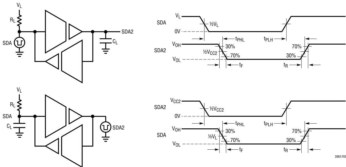
Figure 3. I²C Timing Measurements
