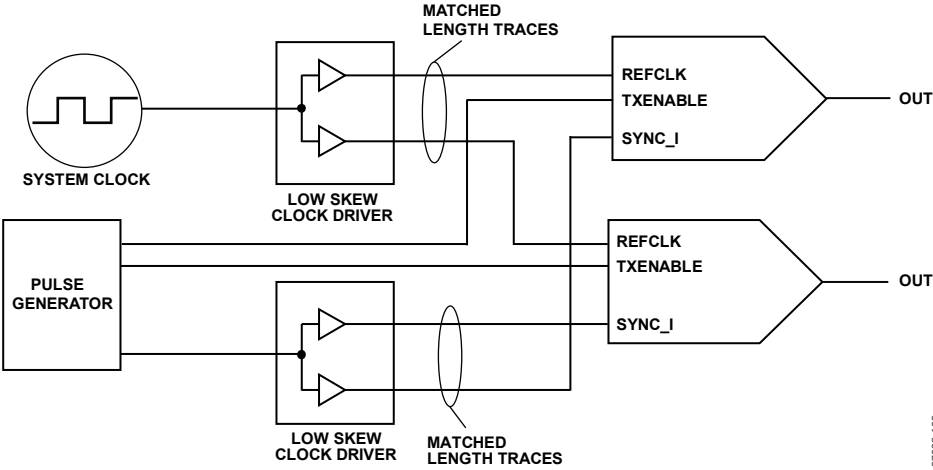
Figure 61. Multichip Synchronization in Pulse Mode
