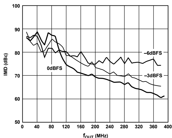
Figure 24. AD9788 IMD Performance vs. Digital Full-Scale Input, 4x Interpolation, f_{DATA} = 200 MSPS
