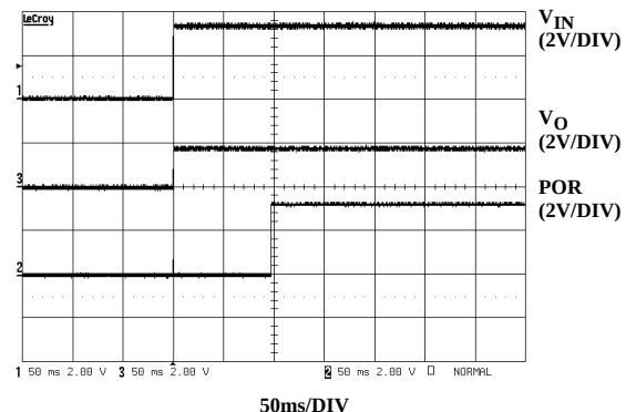
FIGURE 6. START-UP 2
