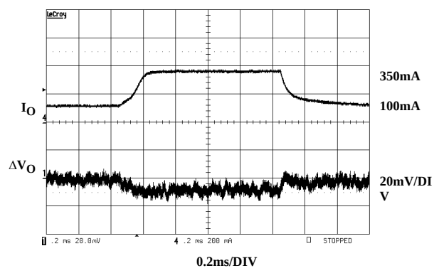
FIGURE 8. TRANSIENT RESPONSE
