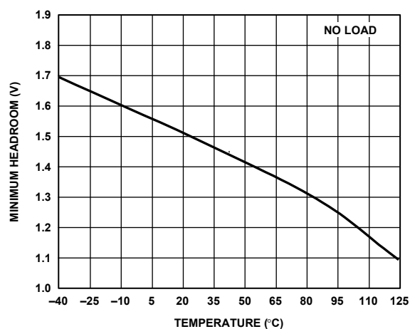
Figure 13. ADR431 Minimum Headroom vs. Temperature
