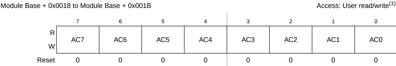
Figure 8-21. MSCAN Identifier Acceptance Registers (Second Bank) — CANIDAR4–CANIDAR7
