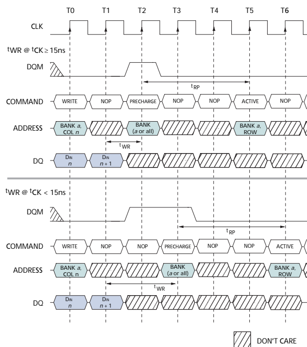
Figure 21: WRITE-to-PRECHARGE
