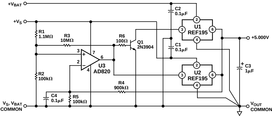
Figure 24. A Fail-Safe 5 V Reference
