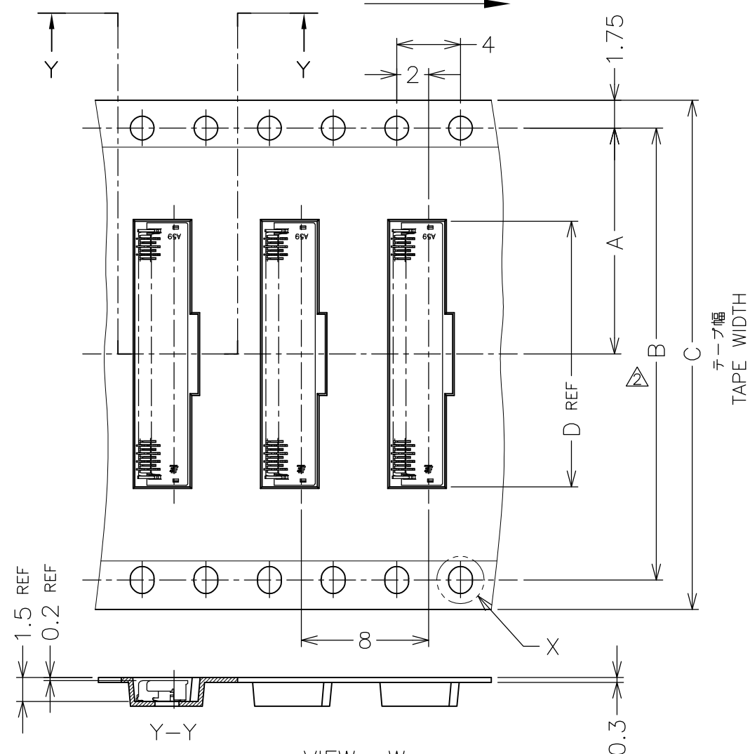
VIEW W
