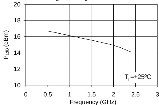
P 1dB vs. Frequency V_D = 3.6\text{ V} , I_D = 60\text{ mA (Typ.)}
