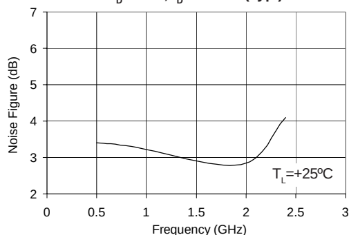
Noise Figure vs. Frequency V_D = 3.6\text{ V} , I_D = 60\text{ mA (Typ.)}
