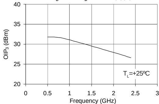
OIP 3 vs. Frequency V_D = 3.6\text{ V} , I_D = 60\text{ mA (Typ.)}
