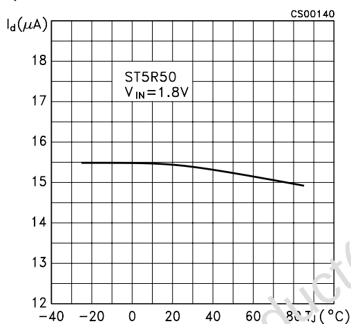
Figure 31: No Load Input Current vs Temperature
