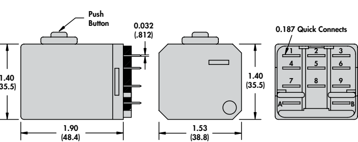
Plug-In Dimensions
