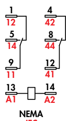
Wiring Diagram Bottom View
