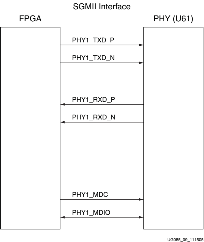
Figure 2-9: SGMII Interface
