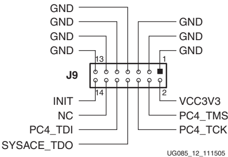
Figure 2-12: PC4 JTAG Connector Pinout (J9)
