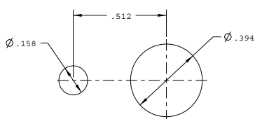
PANEL LAYOUT
