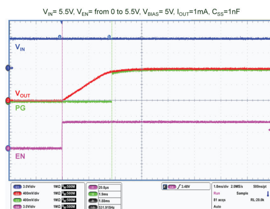
Figure 19. Turn-on time ( C_{SS} = 1 \text{ nF} )
