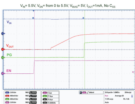
Figure 18. Turn-on time ( C_{SS} = 0 nF)
