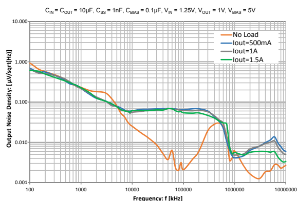
Figure 15. Noise spectral density
