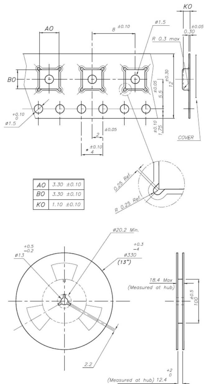
Figure 24. DFN10 (3x3 mm) tape and reel
