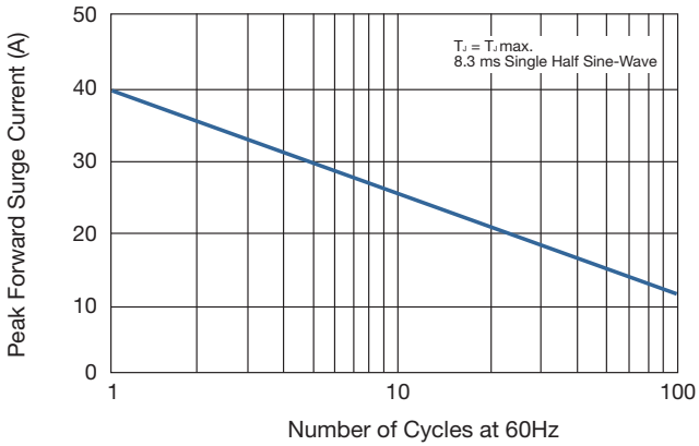
FIG 2. MAXIMUM NON-REPETITIVE
