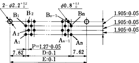
Mating Side
