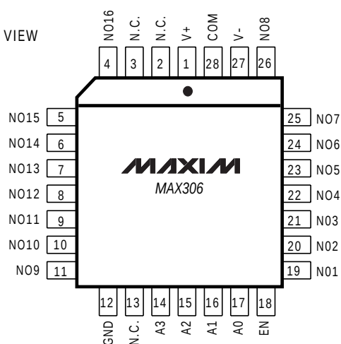
PLCC
