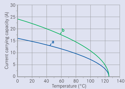
Curve b: 2.5 mm² wire gauge
