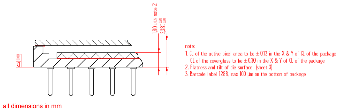
Figure 15. Tolerances
