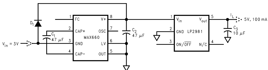
FIGURE 10. Generating +5V from +3V Input Voltage
