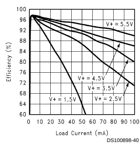
Efficiency vs Load Load Current
