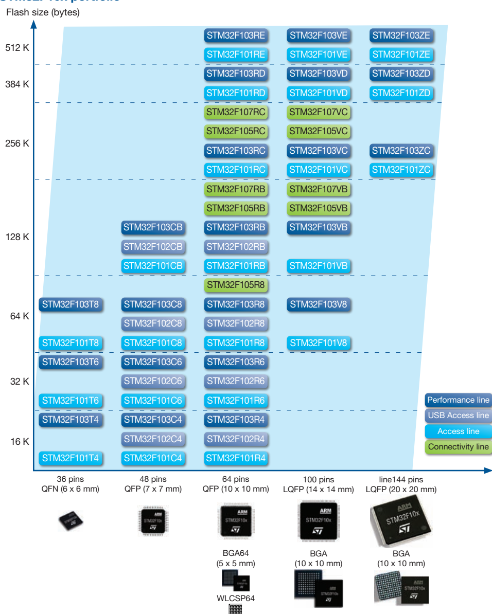
STM32F10x portfolio
