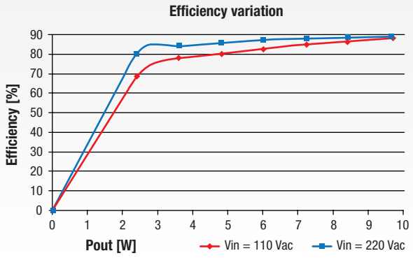
Application example: flyback SMPS for offline LED driver
