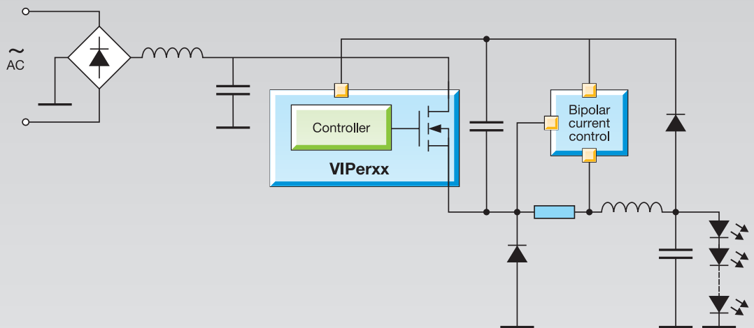
Application example: buck SMPS offline LED driver (non isolated)
