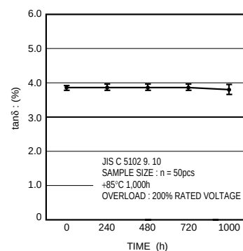
Fig.23 tanδ
