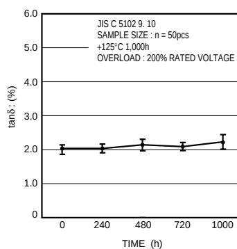
Fig.20 tanδ
