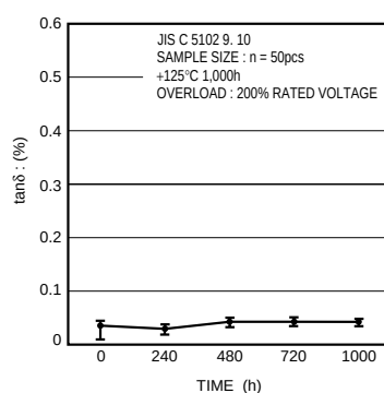
Fig.17 tanδ
