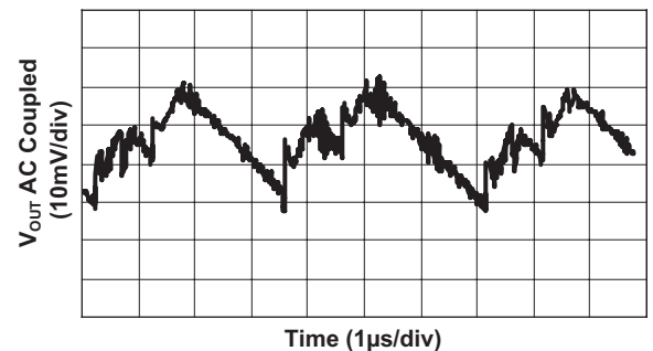
Output Ripple ( I_{OUT} = 100mA ; V_{IN} = 2.5V )
