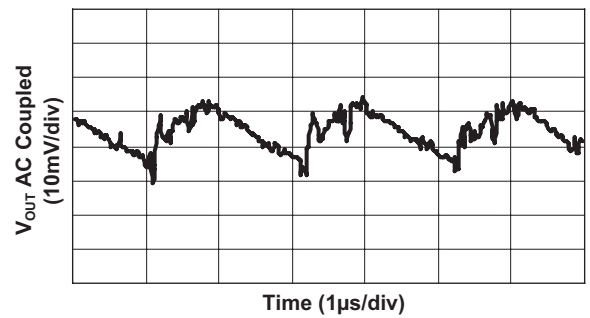
Output Ripple ( I_{OUT} = 100mA ; V_{IN} = 3.0V )
