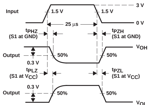
VOLTAGE WAVEFORMS
