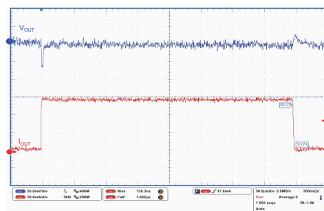
Figure 45. Load transient ( I_{OUT} = 1 to 300 \text{ mA} , normal mode)
