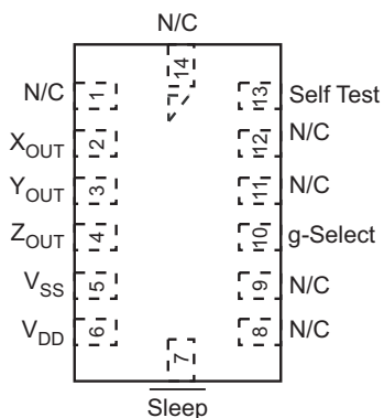
Figure 4. Pinout Description
