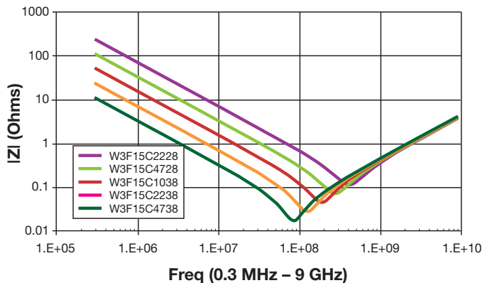
IMPEDANCE 1206 – 50V
