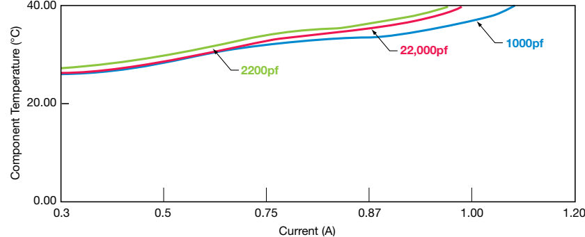
1206 X7R Current vs. Temperature
