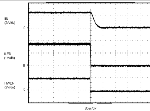
Figure 20. NTC-Mode Operation
