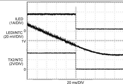
Figure 20. NTC-Mode Operation
