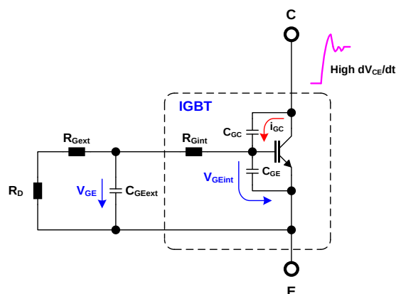
Figure 53. Equivalent circuit of the gate drive
