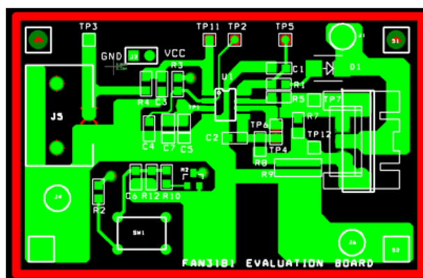
Figure 57. Top View
