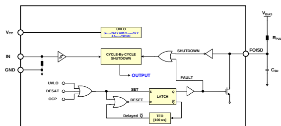
Figure 43. Application Circuit of Fault-Out
