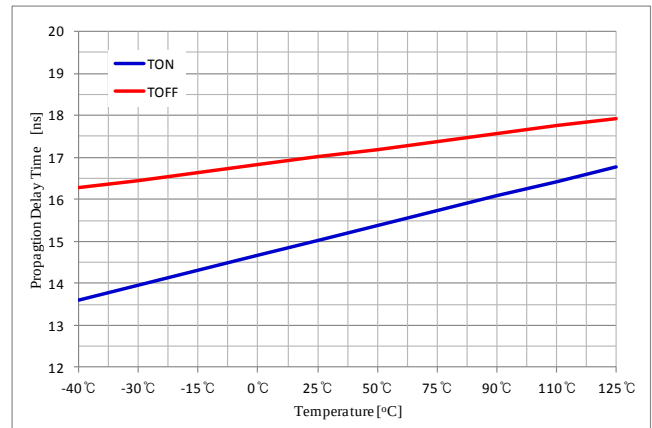
Figure 14. Propagation Delay Time vs. Temperature
