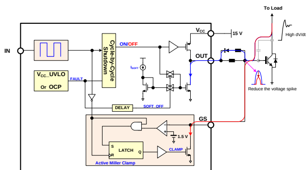
Figure 54. Schematic of Active Miller Clamp
