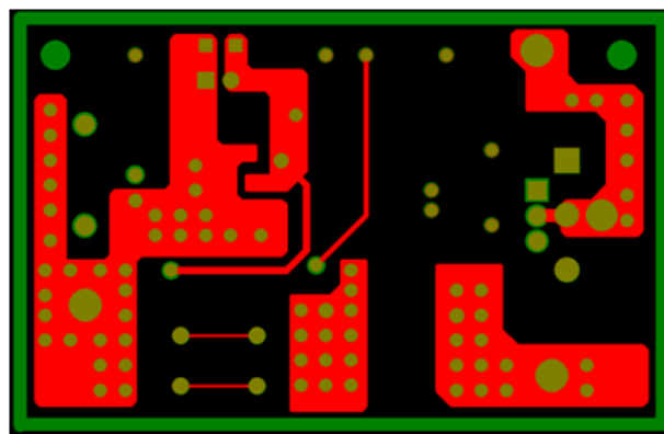
Figure 58. Bottom View
