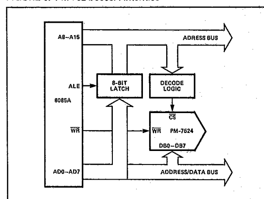
FIGURE 6: PM-7524/8085A Interface
