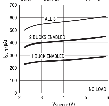
I_{\text{SVIN}} vs V_{\text{SUPPLY}} Pulse-Skipping
