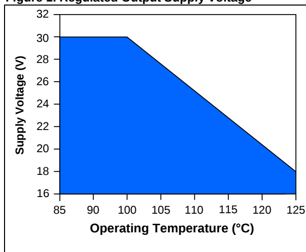
Figure 1. Regulated Output Supply Voltage
