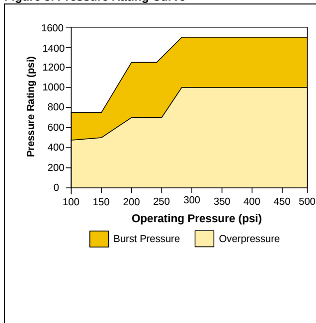
Figure 3. Pressure Rating Curve
