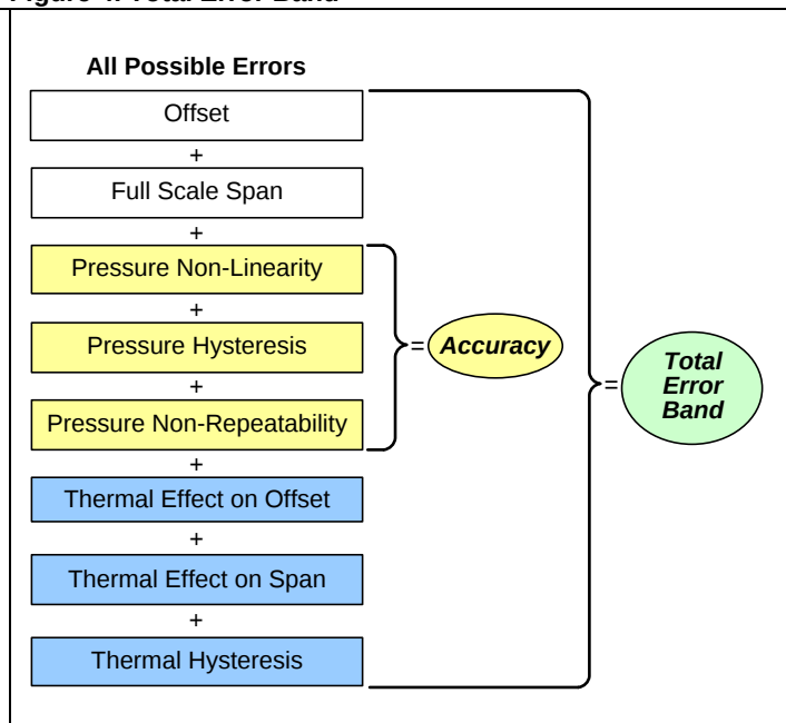
Figure 4. Total Error Band
